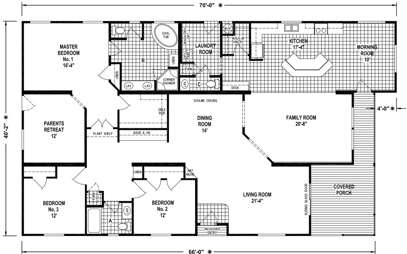
B367CT/7042 (2,479 SQ. FT.) 3BEDROOM • 2 1/2 BATHS
