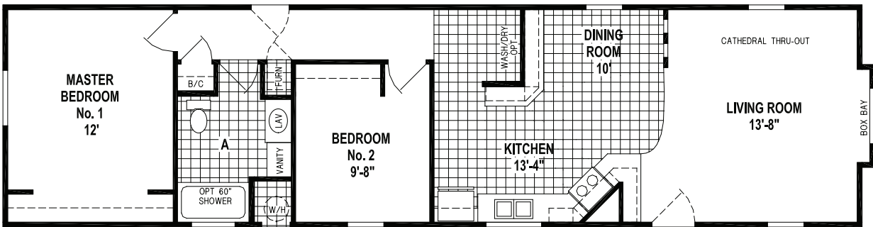
1141CT/6016 (936 SQ. FT.) 2BEDROOM - CATHEDRAL THRU-OUT
